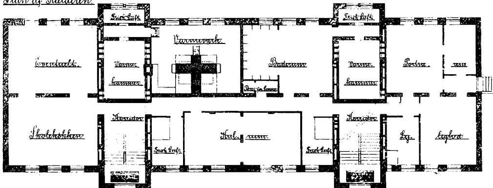
Plan of School
