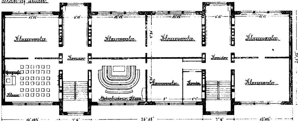
Plan of Ground
