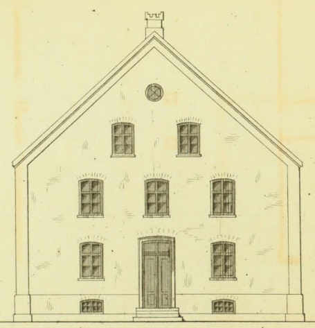
Garbfacade.
