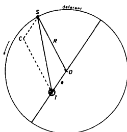
Hipparchus' excentriske model
